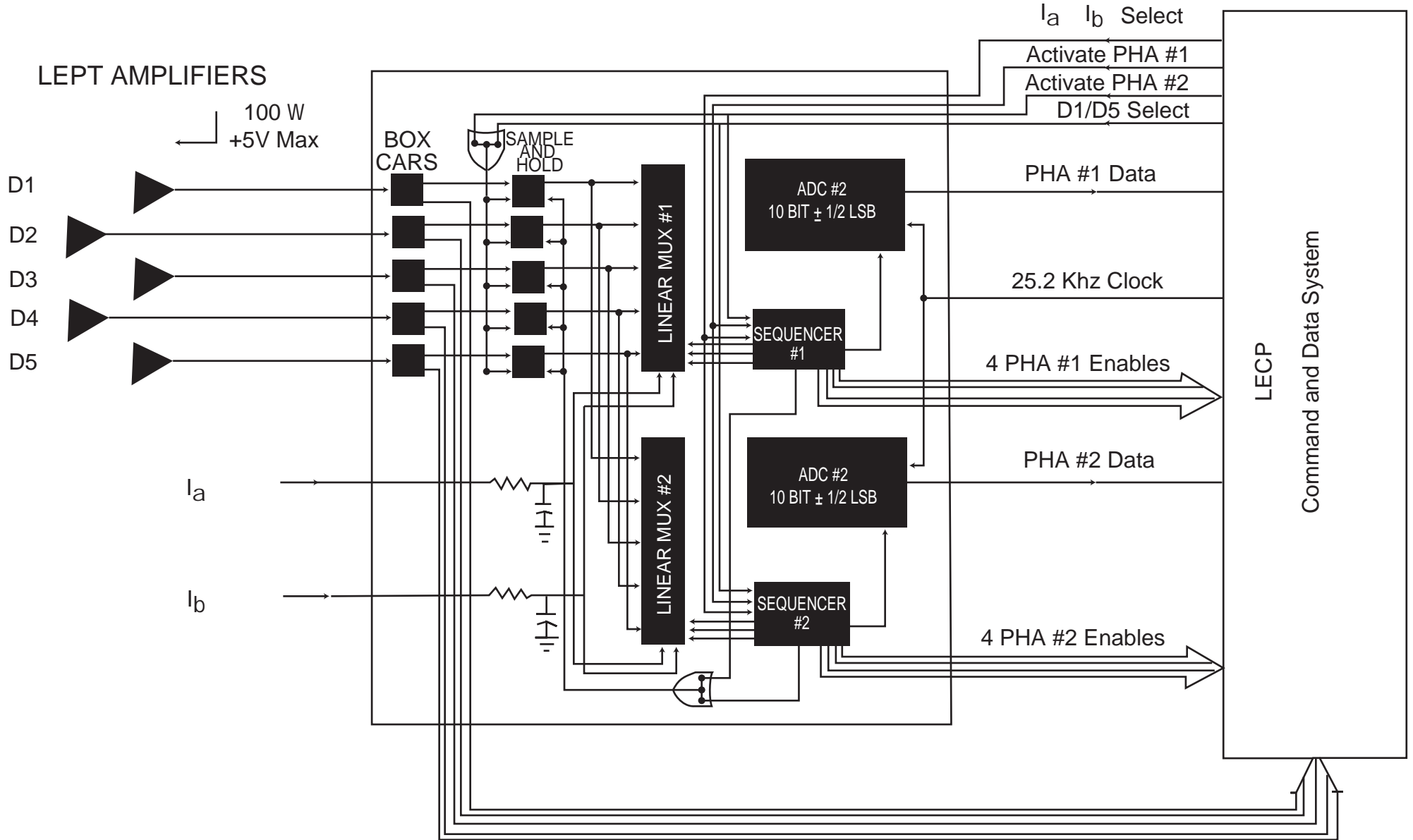
FIGURE 1 LECP PULSE HEIGHT ANALYZER BLOCK DIAGRAM
