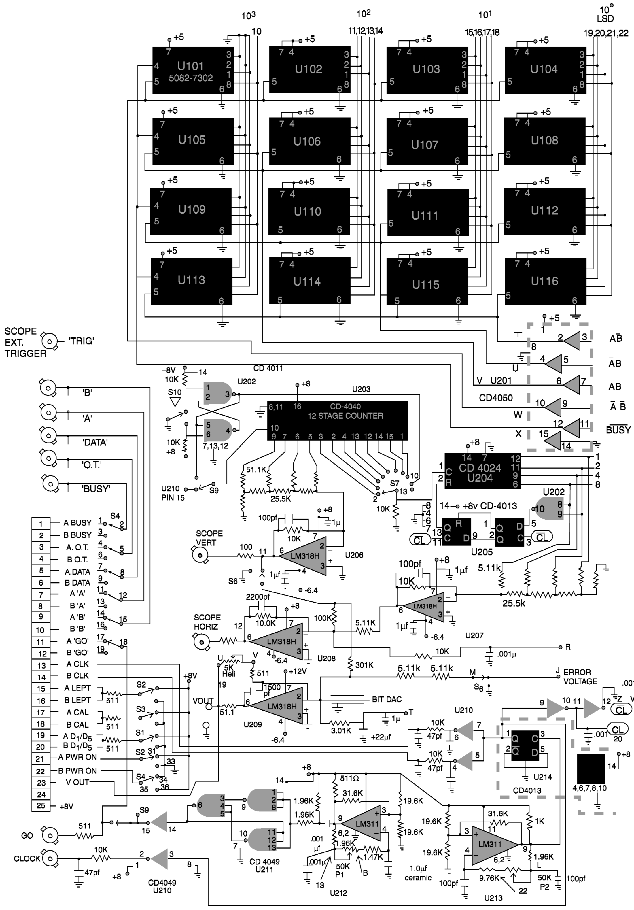
A-5 PHA TEST SET - DISPLAY & CONTROL LOGIC
