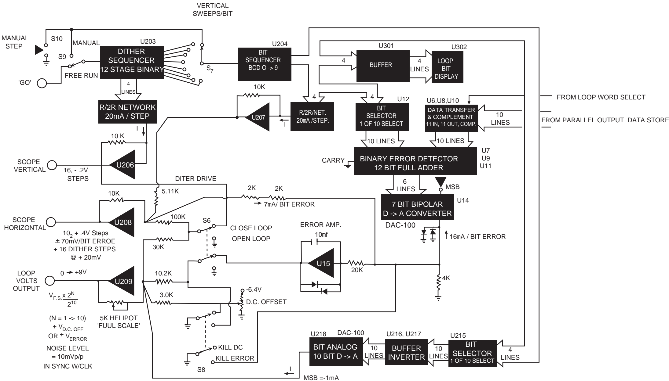
A-2 PHA TEST SET - DIGITAL SERVO CONTROL LOOP
